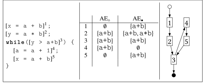
Figure 2: An illustration of available expressions (AE) analysis. On the left is an example program in the WHILE language, with added brackets to number program fragments. On the right is the control flow graph (CFG) of the program. In the center is the analysis result. The open and closed dots on the analysis abbreviation are before and after a CFG node's effect respectively.
