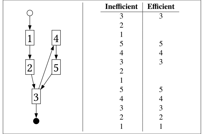
Figure 25: An illustration of efficient and inefficient order in a backward analysis that requires two round through loop 3,4,5 before reaching a fixed point. The inefficient order always propagates from 3 to 2,1 first, whereas the efficient order first propagates from 3 to 5,4.
