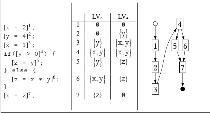
Figure 1: An illustration of live variables (LV) analysis. On the left is an example program in the WHILE language, with added brackets to number program fragments. On the right is the control flow graph (CFG) of the program. In the center is the analysis result. The LV o and LV • are respectively before and after the variable accesses of the CFG node.
