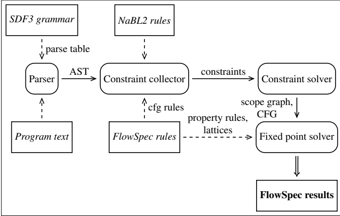
Figure 24: Architecture diagram of FlowSpec within the context of the Spoofox language workbench. A program from an object language is first parsed using a grammar in SDF3. Then we use a NaBL2 static semantics definition to analyze the names and types in the program. The same machinery is used to build the control flow graph, based on the FlowSpec control flow graph rules. A separate fixed point solver is the new addition that computes data-flow information based on the FlowSpec specification.
